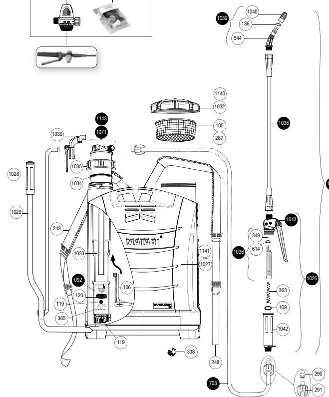
1 M - 39.37 INCH ALUMINIUM LANCE TUBE WITH COMPLETE ELBOW Reference 8.34.60.871 1,5 M - 59 INCH ALUMINIUM LANCE TUBE WITH COMPLETE ELBOW Reference 8.34.60.872
